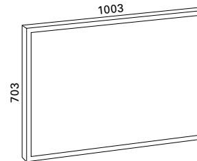
EVO 100X70 • mitat L1003 x K703 x S38 mm
